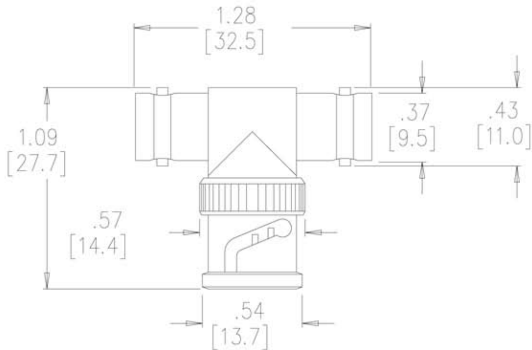
JACK-PLUG-JACK
