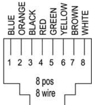
WIRING BACK VIEW 8 POS 8 COND
