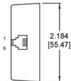
WIRING VIEW
