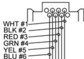
WIRING VIEW
